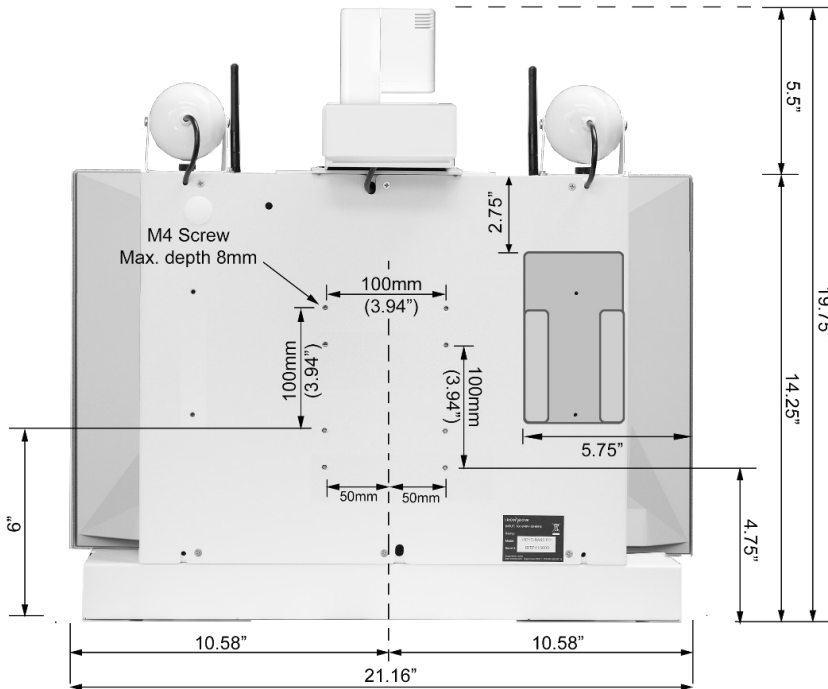
Rear System Dimensions
